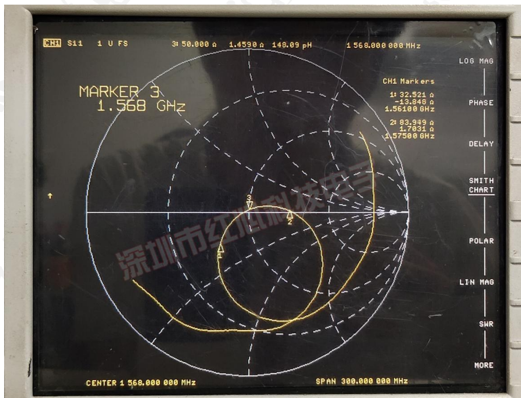
Smith Chart (史密斯圆图)
