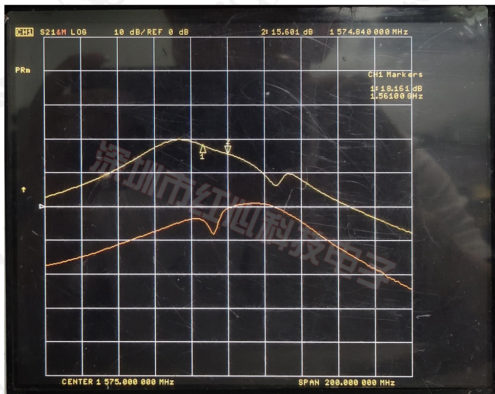
(Gain)增益图
