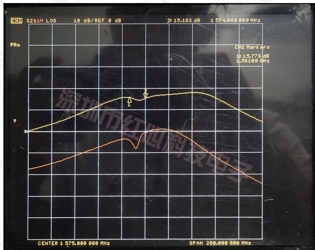
(Gain)增益图
