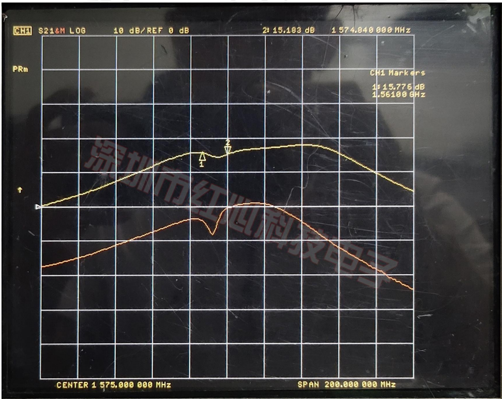
(Gain)增益图
