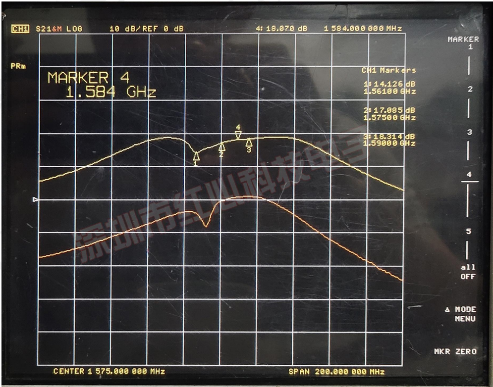
(Gain)增益图
