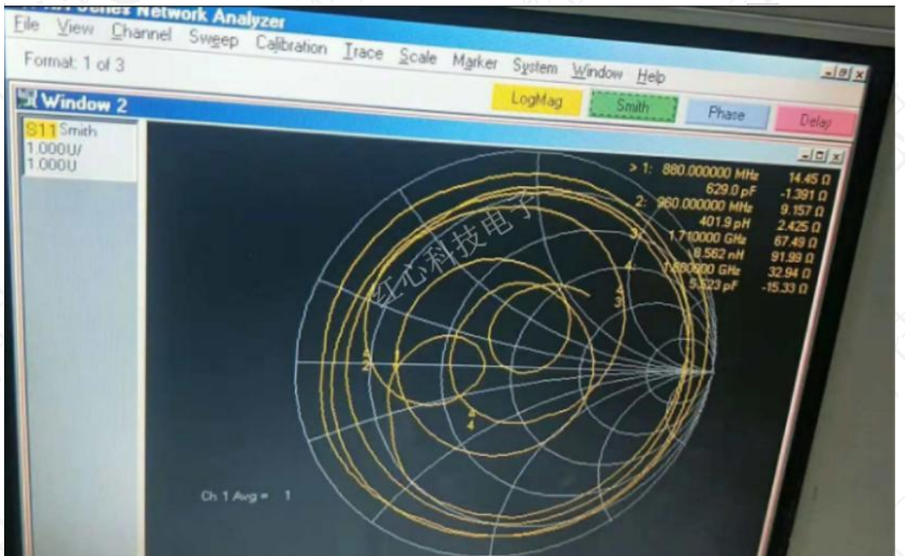
Smith Chart (史密斯圆图)
